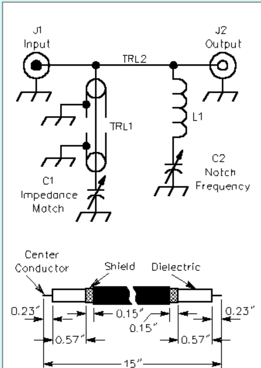
TRL1 End Detail
