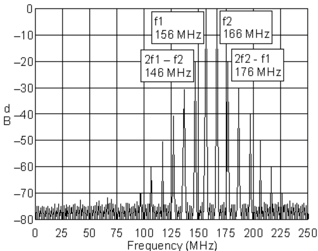
Figure 3--These pager frequencies can intermodulate to form a product in the amateur 2-meter band. If there are many pagers on different frequencies in the same area, the result can be interference across the band. This actually occurs in some major cities. This graph shows third- and higher odd-order products.
