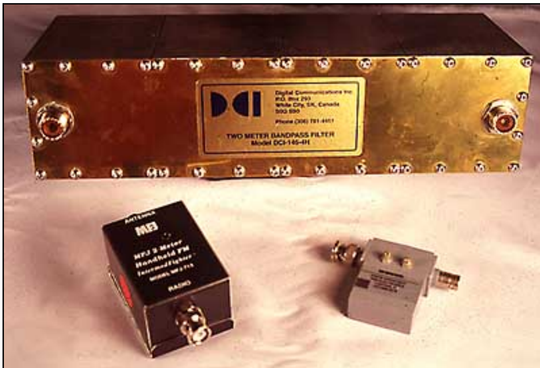
Figure 5--Two of the three shown are band-pass filters . One of them is a notch filter . All three are commercial.
