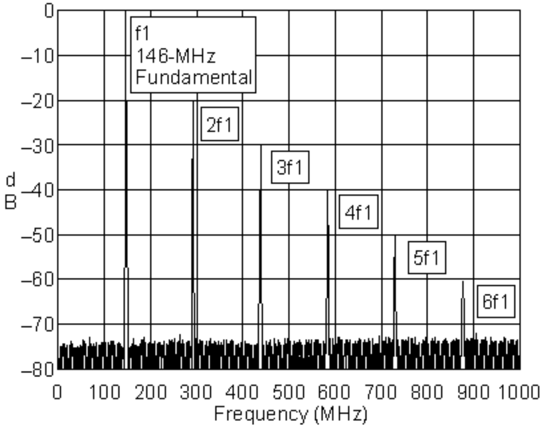
Figure 1--This 146-MHz signal contains harmonics that extend well into the UHF range.
