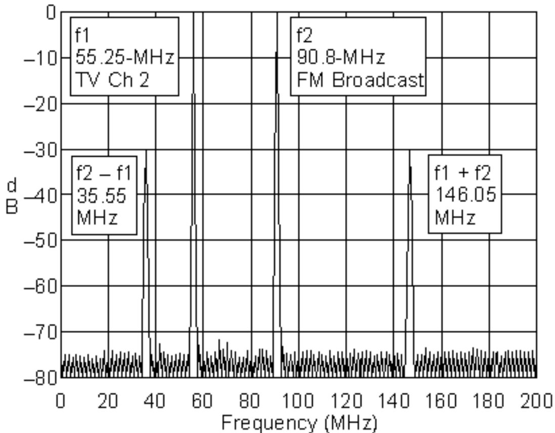
Figure 2--Here, f1 (55.25 MHz) and f2 (90.8 MHz) are present at the input of a VHF receiver, they may generate an interfering signal (f1 + f2) on 146.05 MHz.
