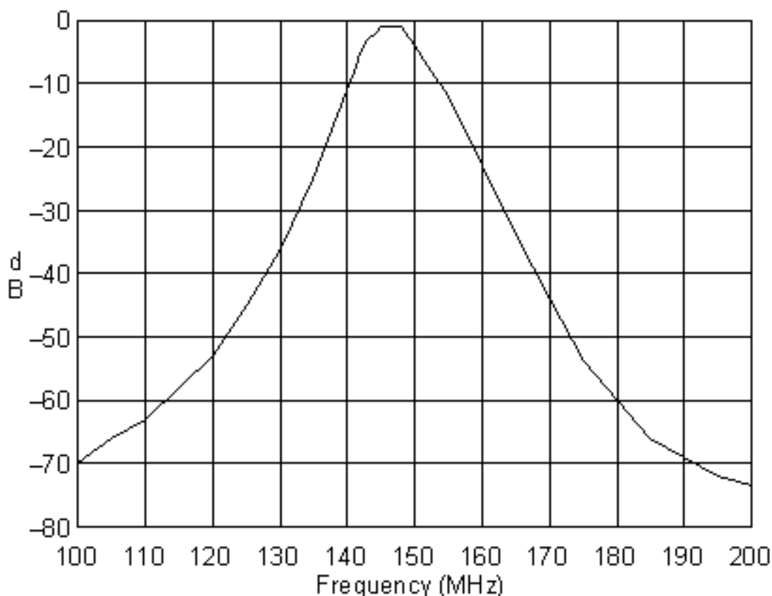
Figure 6--The frequency response of a typical band-pass filter. This filter's passband centers near 147 MHz. Its 3-dB bandwidth is about 7 MHz (143 to 150 MHz).
