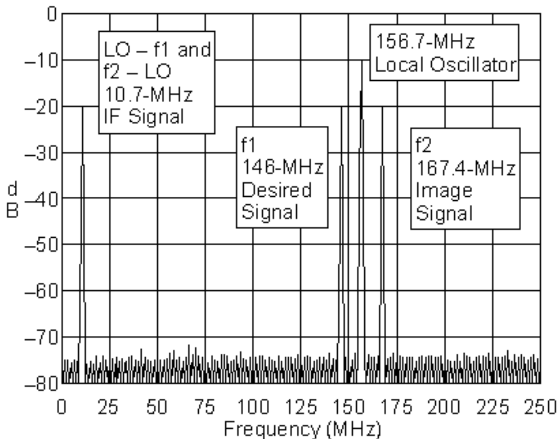
Figure 4--A superheterodyne receiver can respond to signals other than the desired signal. If the RF selectivity of the receiver is inadequate (poor image rejection), the receiver could hear the signal on 167.4 MHz in addition to the desired signal on 146 MHz.
