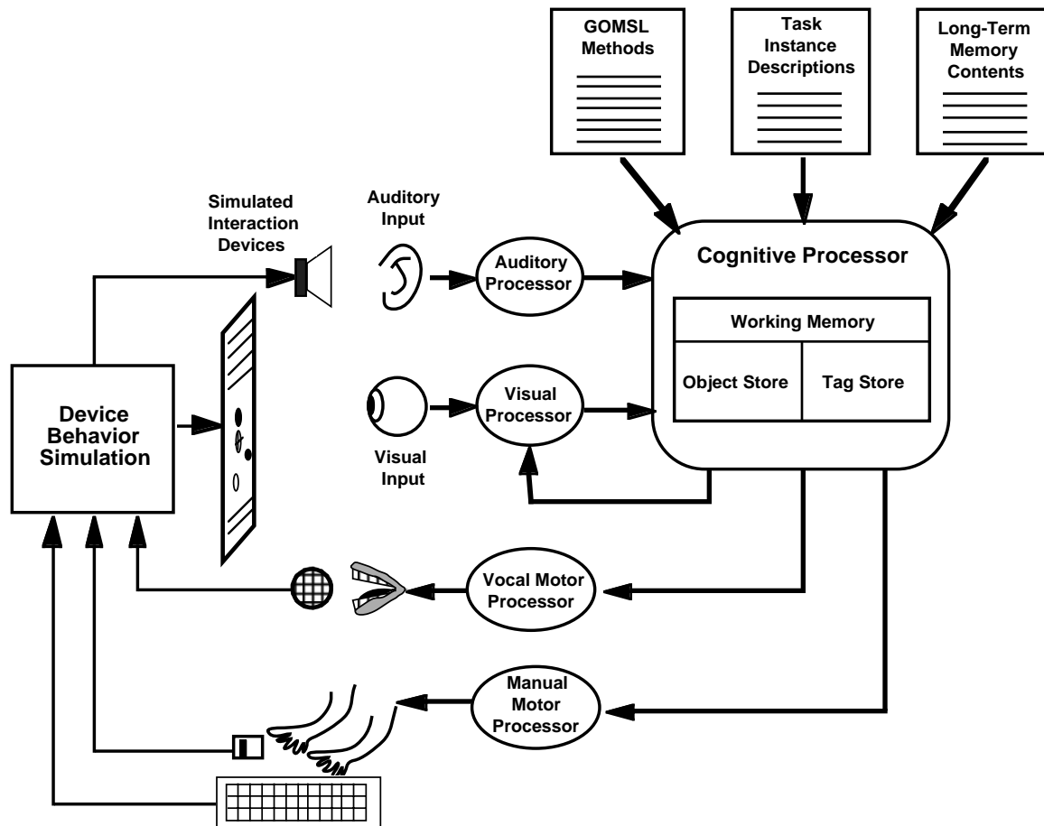
Figure 1. The GLEAN3 architecture.
